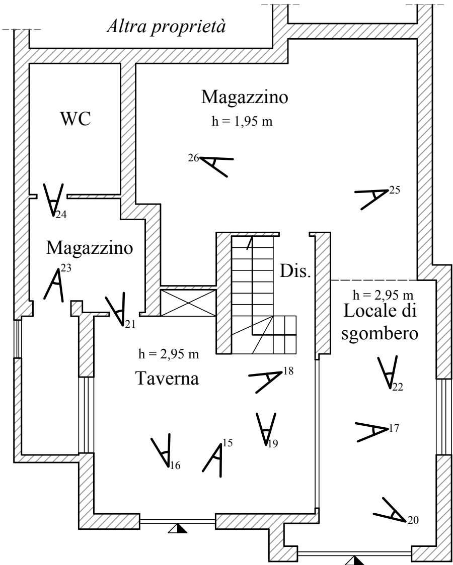
PIANO SEMINTERRATO SCALA 1:100
