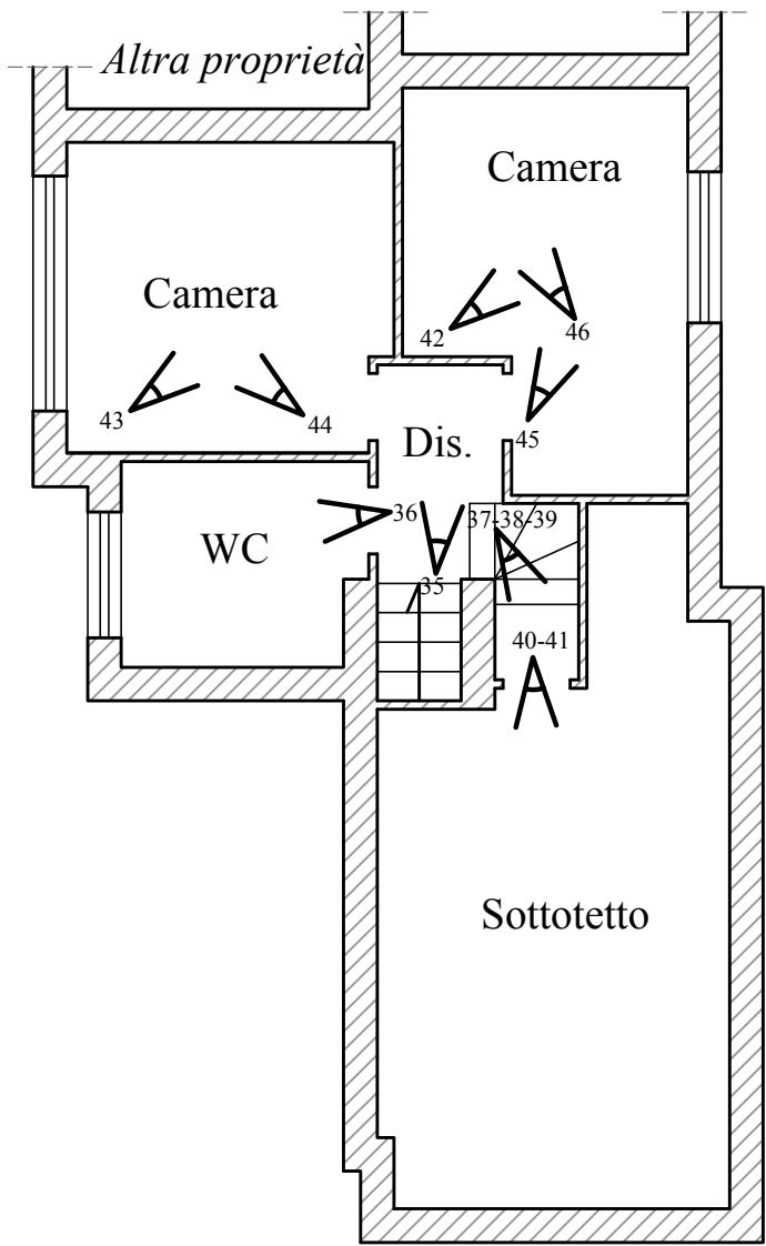
PIANO MANSARDA SCALA 1:100
